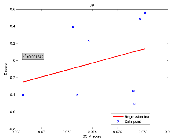
Figure 20. Regression line plot SSIM for JP data points
