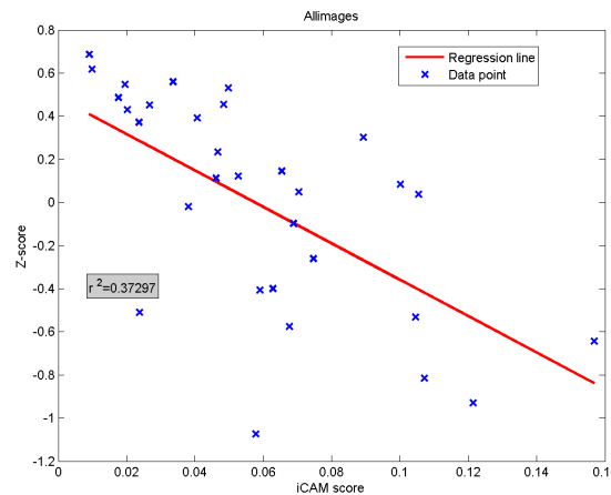
Figure 18. Regression plot for iCAM weighted with eye tracker map
