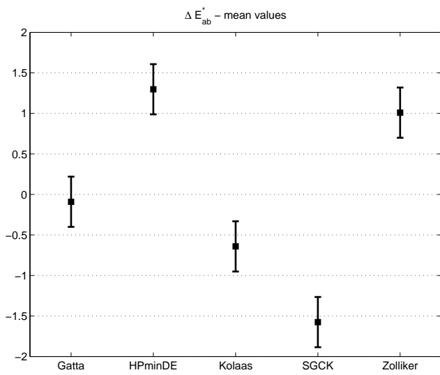
(a) \Delta E_{ab}^* rank order score.
