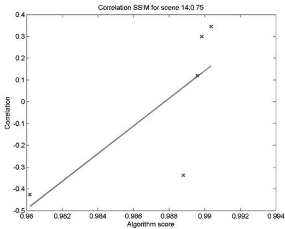
Figure 6. Correlation between z-score and calculated image difference for SSIM on scene 14. The visual difference between the images is not correctly predicted by SSIM, but the ranking is. Based on this the rank order method on the SSIM data will be a better measure.
