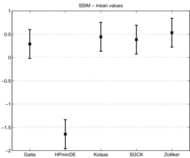
(a) SSIM rank order score.
