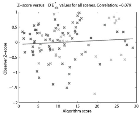
Figure 3. Z-score from observers against \Delta E_{ab}^* values. The data points are very spread, and we get a very low correlation between the z-scores and \Delta E_{ab}^* values. The HPminDE algorithm is rated as the best by \Delta E_{ab}^* the opposite of the observers.
