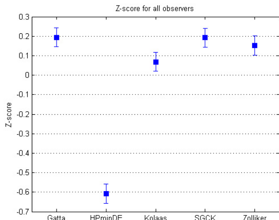
Figure 2. Z-score from pair comparison experiment I. Gatta cannot be differentiated from SGCK and Zolliker. Kolás is rated barely lower than the Gatta, SGCK but cannot be differentiated from Zolliker. HPminDE receives the lowest z-score from the observers.
