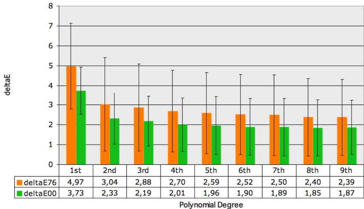
Figure 3. Average performance for direct transformation with varying polynomial order
