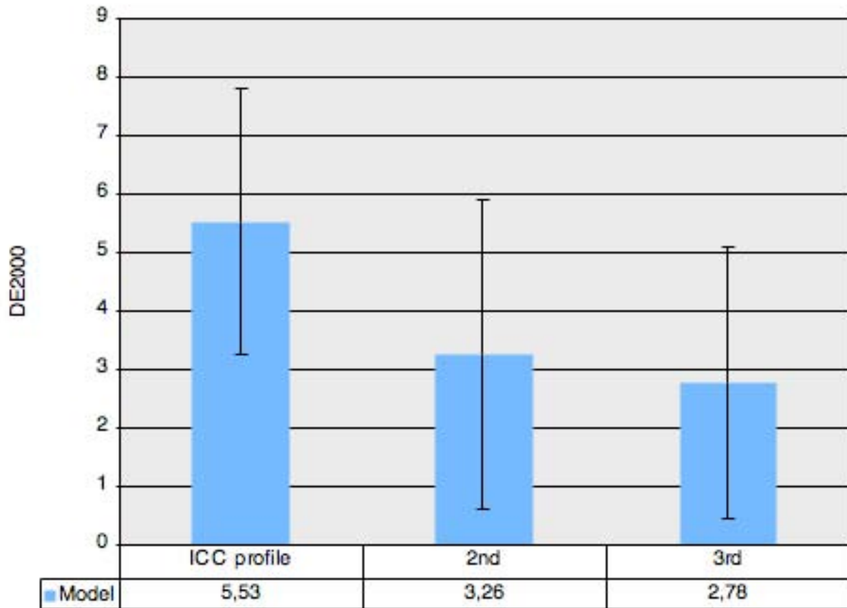
Figure 7. The reverse model of a camera ICC profile compared to a model based on polynomial regression
